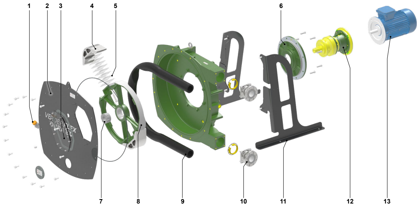
Figure 1. - Layout Dura 80 (Generic View)
